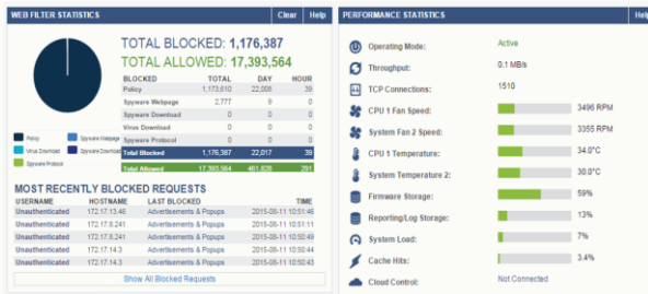
Fig. 2. Performance Statistics
