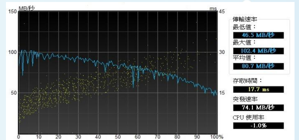
Fig.8 HDD transfer rate
