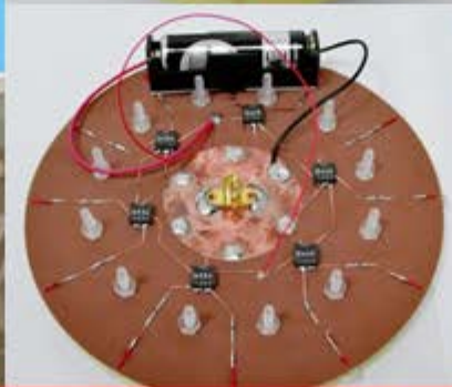
Multi-polarization Circular Patch Antenna
