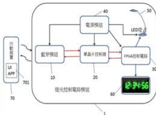
Bluetooth LED Lighting Control System
