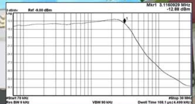
Fig. 4 Measured frequency response of the low-pass filter.
