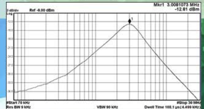
Fig. 3 Measured frequency response of the band-pass filter.
