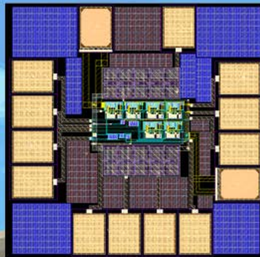
Fig. 2 The layout design of the proposed filter.
